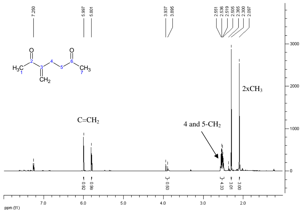
Figure 16: 400MHz ^1\text{H} NMR spectrum of the MVK dimer (3-methyleneheptan-2,6-dione) 30 in \text{CDCl}_3 .
