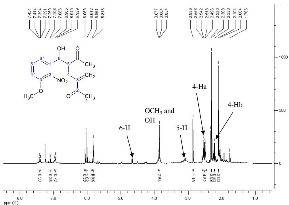
Figure 17: 400MHz ^1\text{H} NMR spectrum of a mixture of the MVK dimer 30 and 5-acetyl-6-(3-methoxy-2-nitrophenyl)-3-methylene-2-hexanone 31e in \text{CDCl}_3 .
