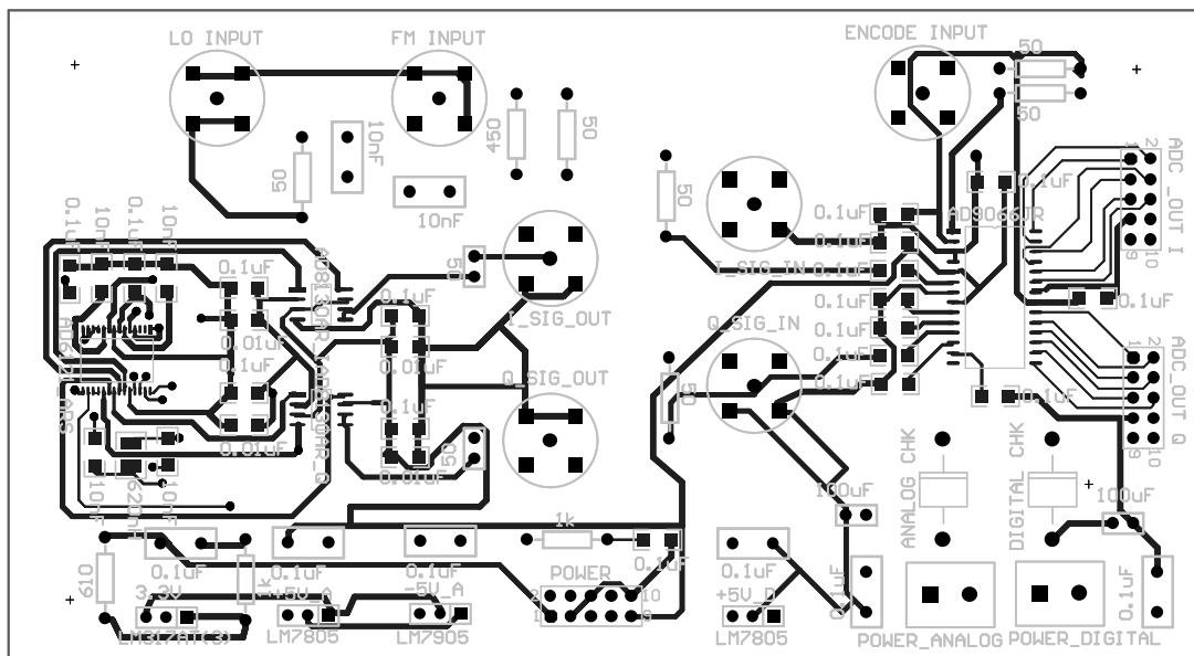
Figure: Printed circuit board of analogue frontend module (Top layer)
