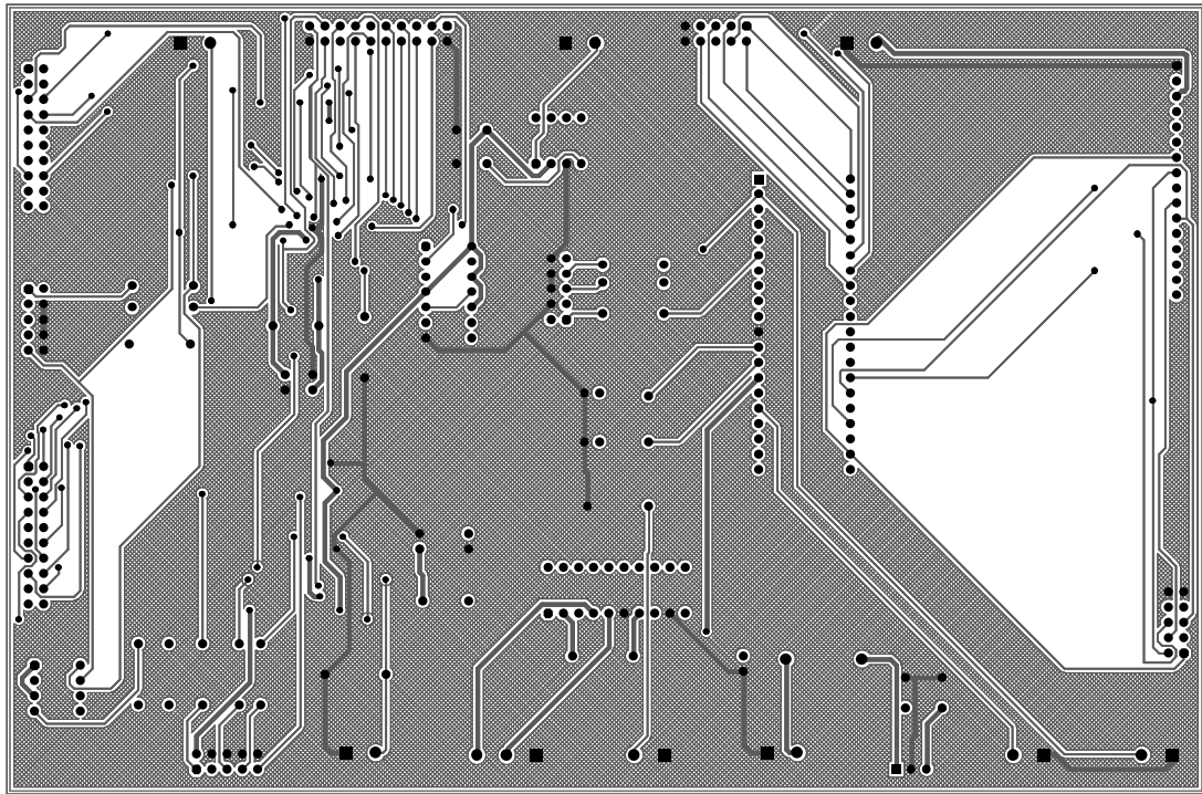
Figure: Printed circuit board of digital backend module (Bottom layer)
